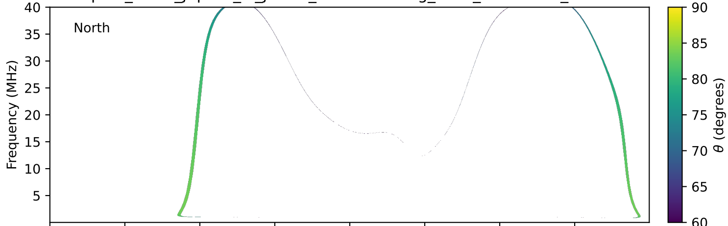
expres_earth_jupiter_io_jrm33_lossc-wid1deg_3kev_19901020_v11.cdf
