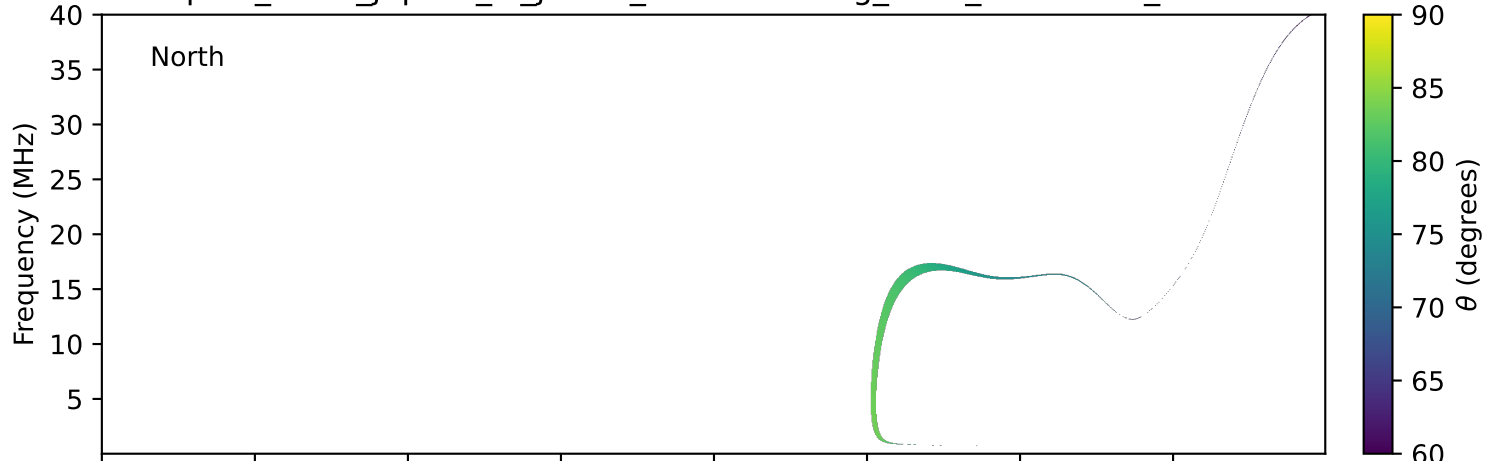
expres_earth_jupiter_io_jrm33_lossc-wid1deg_3kev_19901016_v11.cdf
