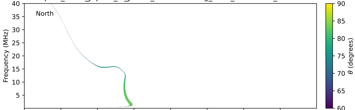
expres_earth_jupiter_io_jrm33_lossc-wid1deg_3kev_19901010_v11.cdf
