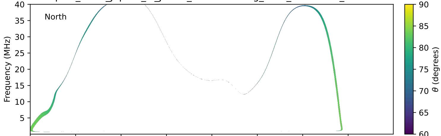
expres_earth_jupiter_io_jrm33_lossc-wid1deg_3kev_19901006_v11.cdf
