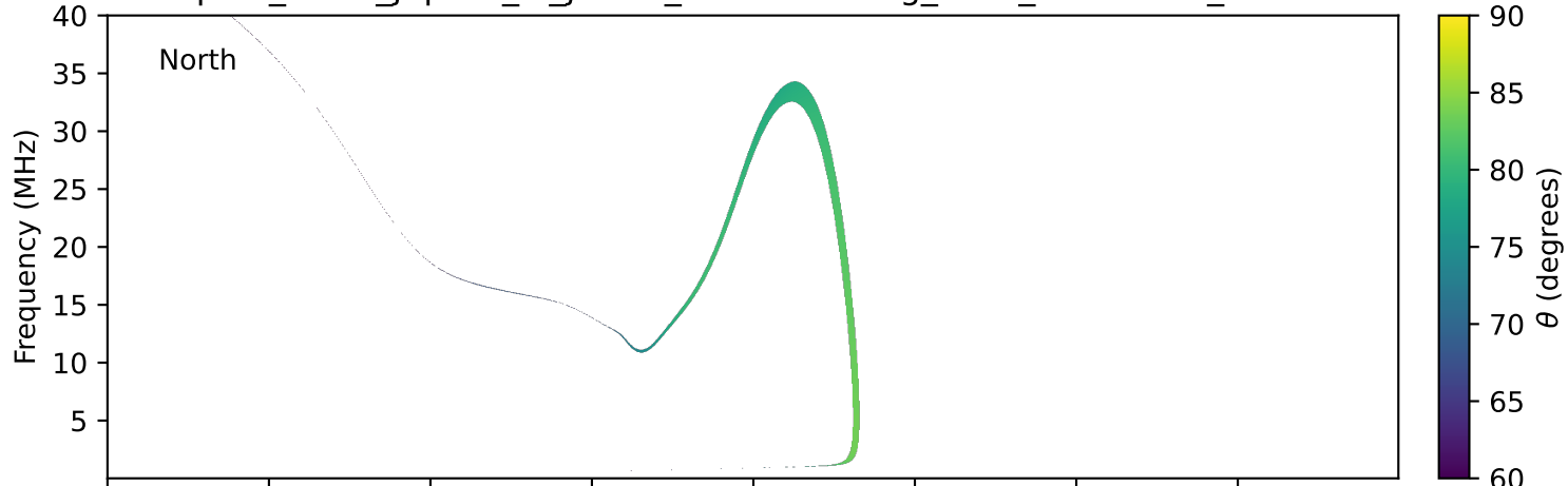
expres_earth_jupiter_io_jrm09_lossc-wid1deg_3kev_19901024_v11.cdf
