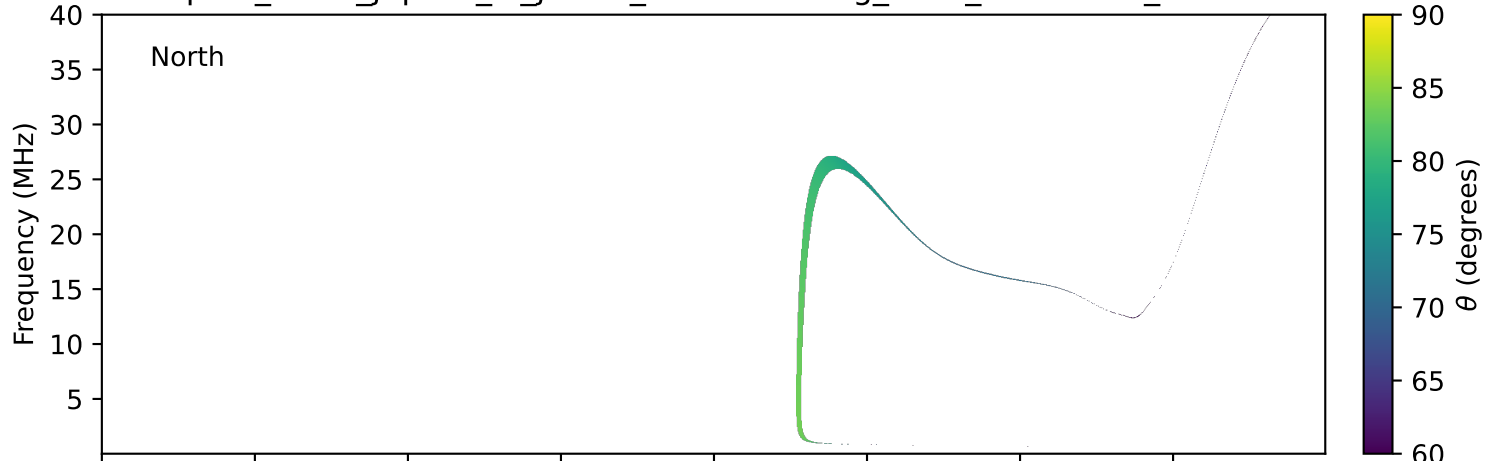
expres_earth_jupiter_io_jrm09_lossc-wid1deg_3kev_19901009_v11.cdf
