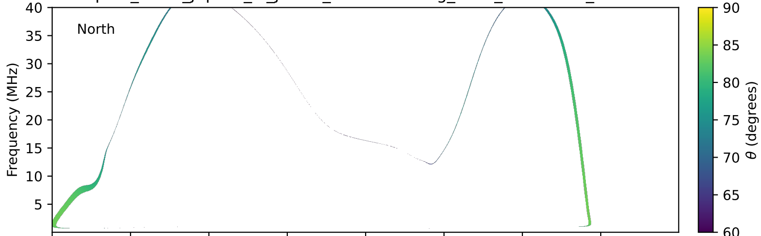
expres_earth_jupiter_io_jrm09_lossc-wid1deg_3kev_19901006_v11.cdf
