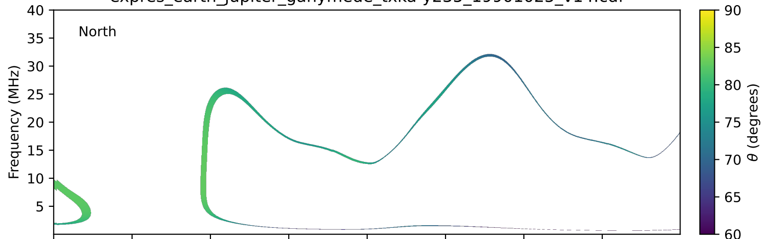
expres_earth_jupiter_ganymede_txka-y235_19901025_v14.cdf
