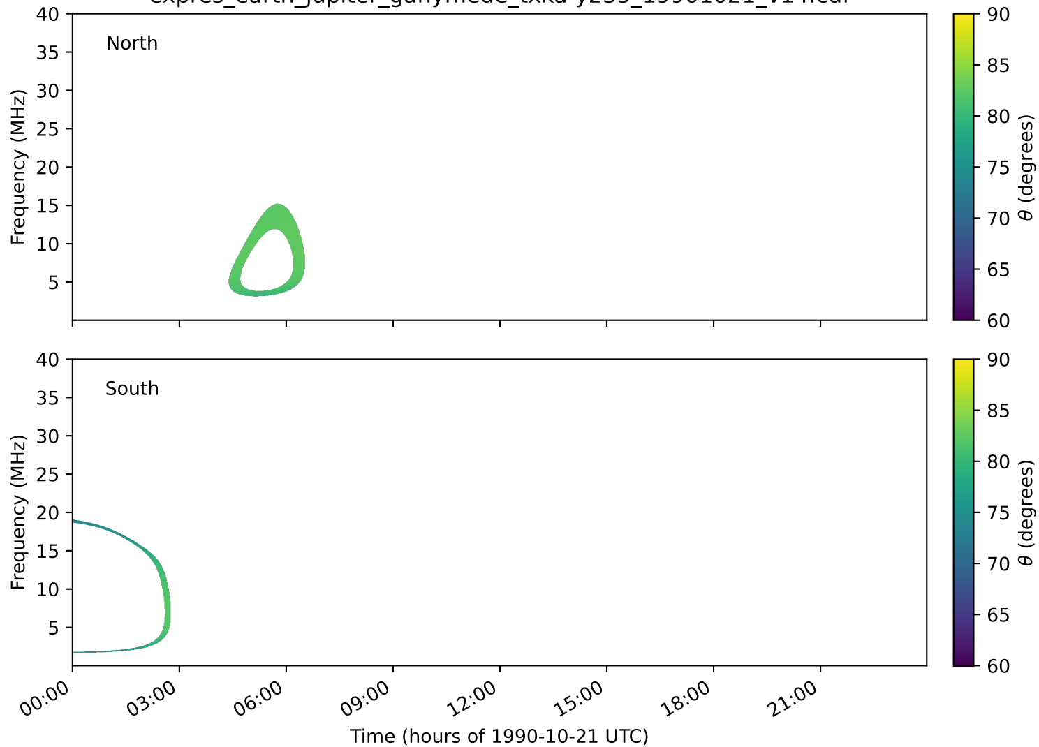
expres_earth_jupiter_ganymede_txka-y235_19901021_v14.cdf
