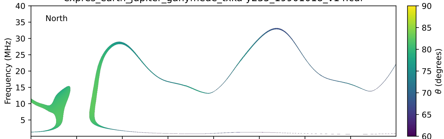
expres_earth_jupiter_ganymede_txka-y235_19901018_v14.cdf
