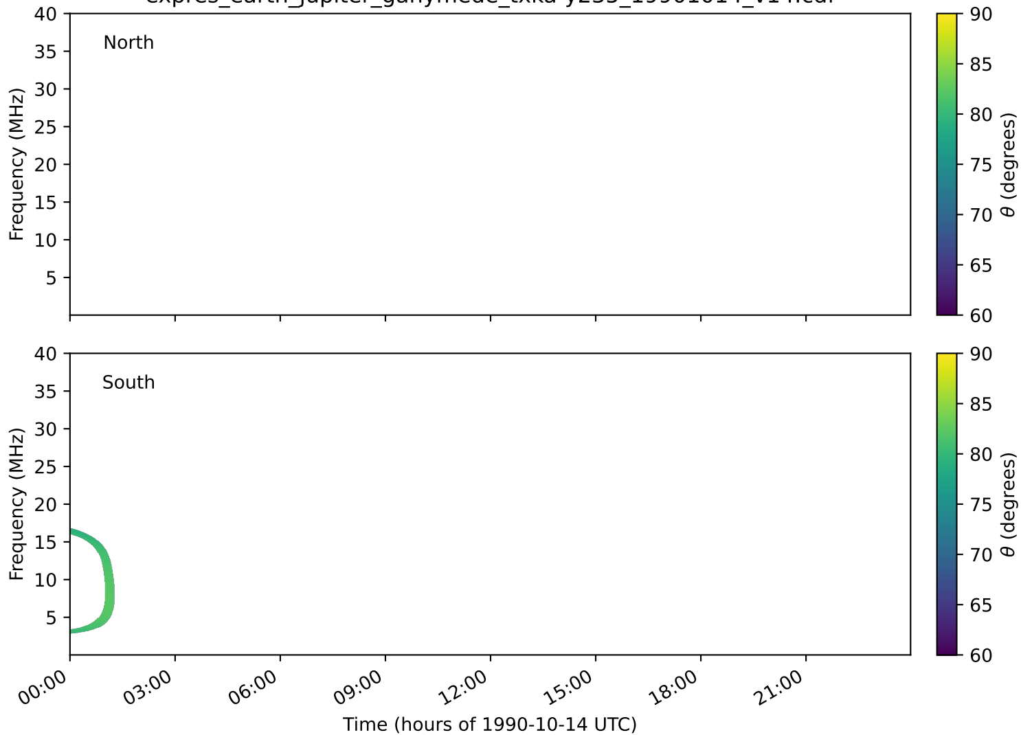
expres_earth_jupiter_ganymede_txka-y235_19901014_v14.cdf
