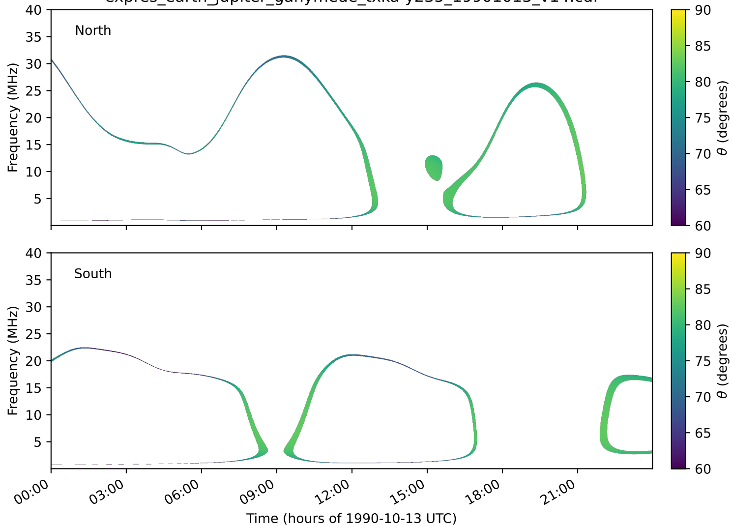
expres_earth_jupiter_ganymede_txka-y235_19901013_v14.cdf
