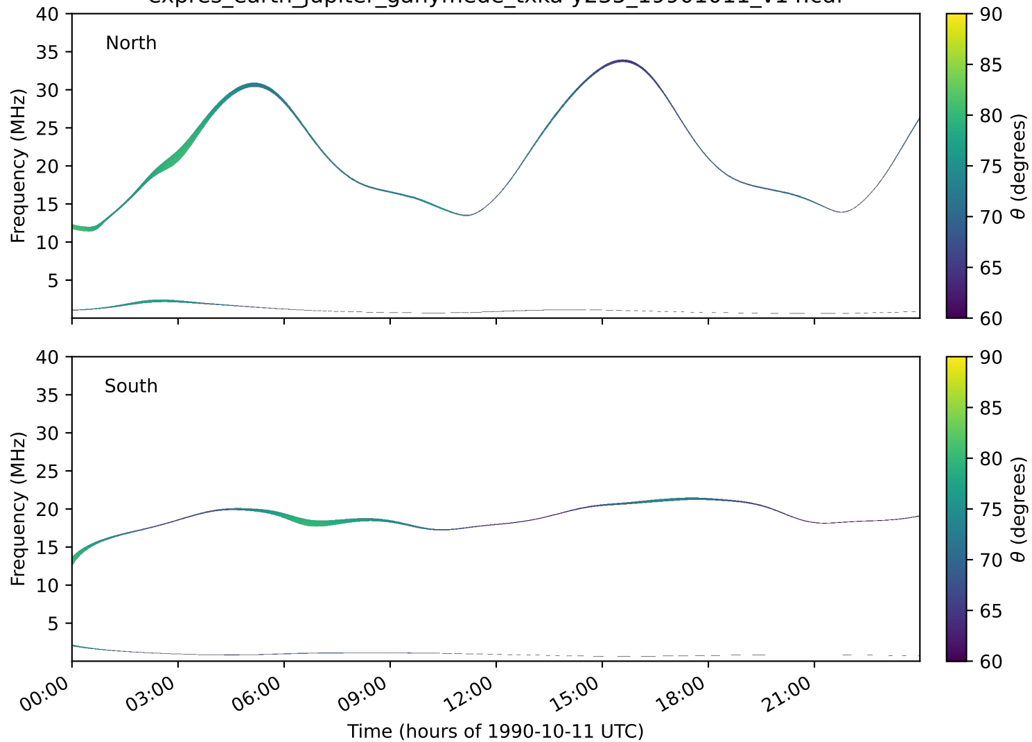
expres_earth_jupiter_ganymede_txka-y235_19901011_v14.cdf
