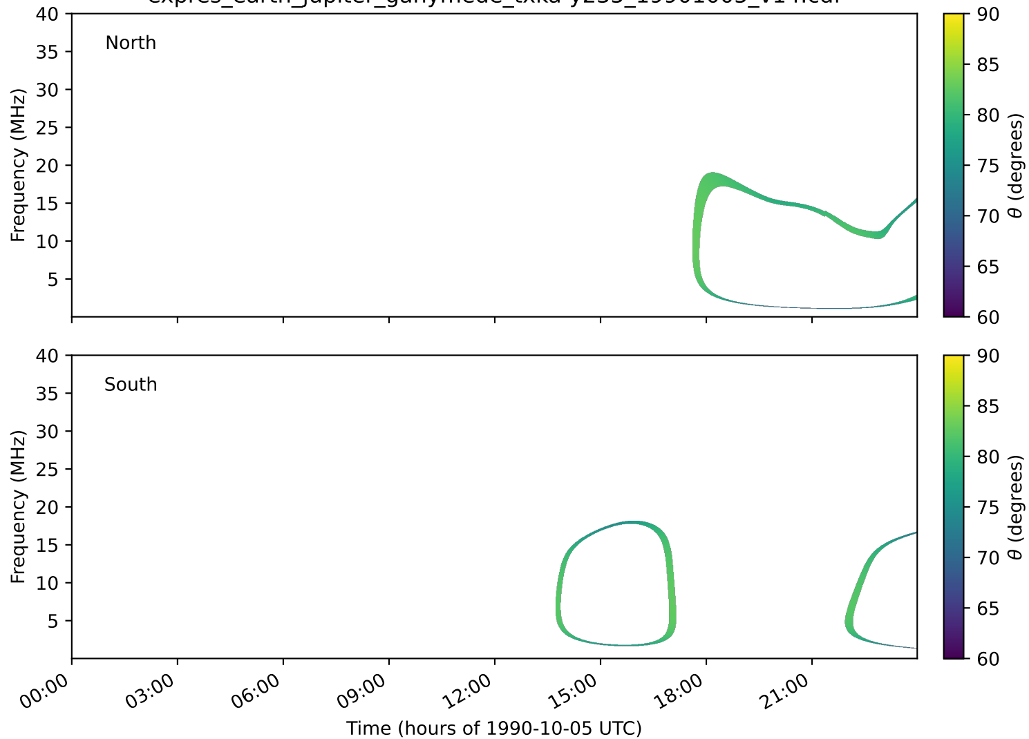
expres_earth_jupiter_ganymede_txka-y235_19901005_v14.cdf
