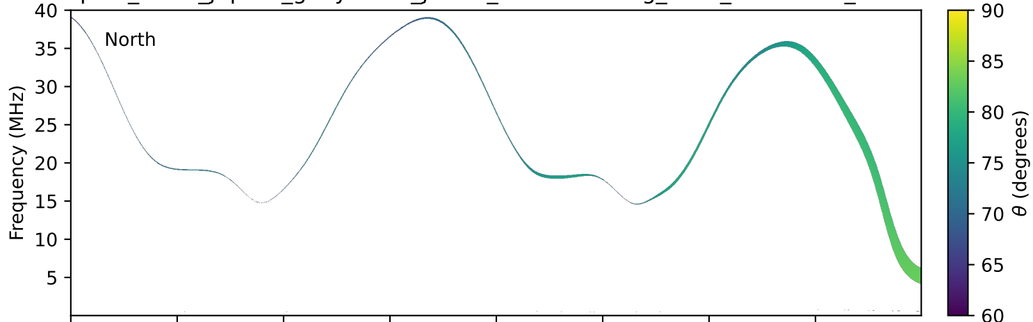
expres_earth_jupiter_ganymede_jrm33_lossc-wid1deg_3kev_19901020_v11.cdf
