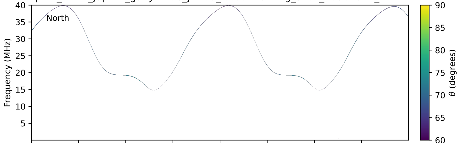
expres_earth_jupiter_ganymede_jrm33_lossc-wid1deg_3kev_19901012_v11.cdf
