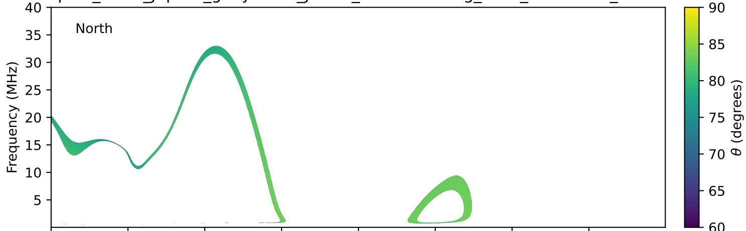
expres_earth_jupiter_ganymede_jrm09_lossc-wid1deg_3kev_19901028_v11.cdf
