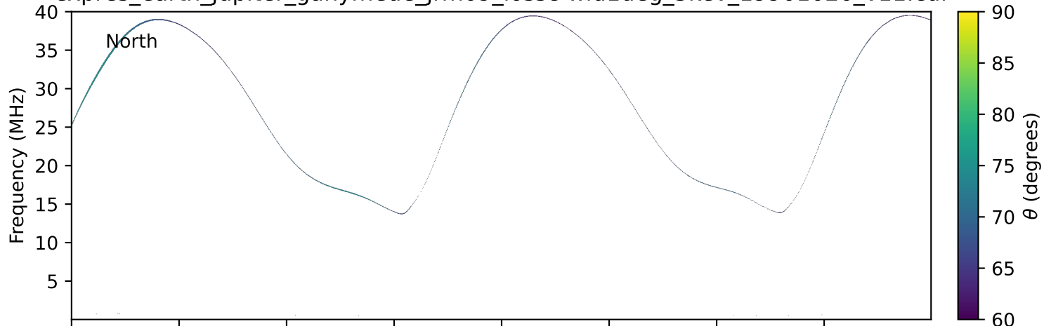
expres_earth_jupiter_ganymede_jrm09_lossc-wid1deg_3kev_19901026_v11.cdf
