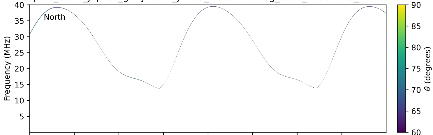
expres_earth_jupiter_ganymede_jrm09_lossc-wid1deg_3kev_19901019_v11.cdf
