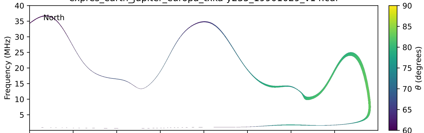
expres_earth_jupiter_europa_txka-y235_19901029_v14.cdf
