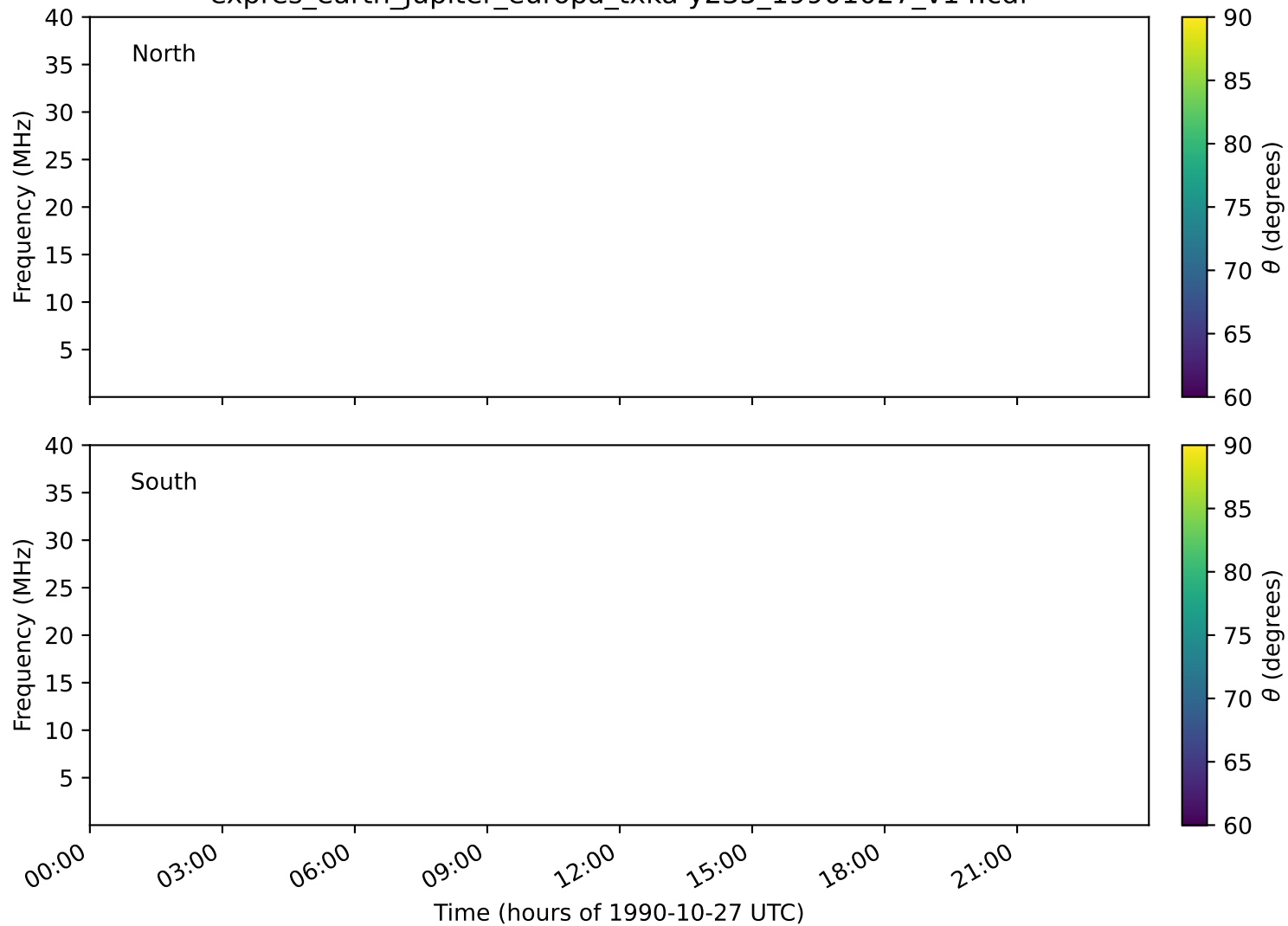
expres_earth_jupiter_europa_txka-y235_19901027_v14.cdf
