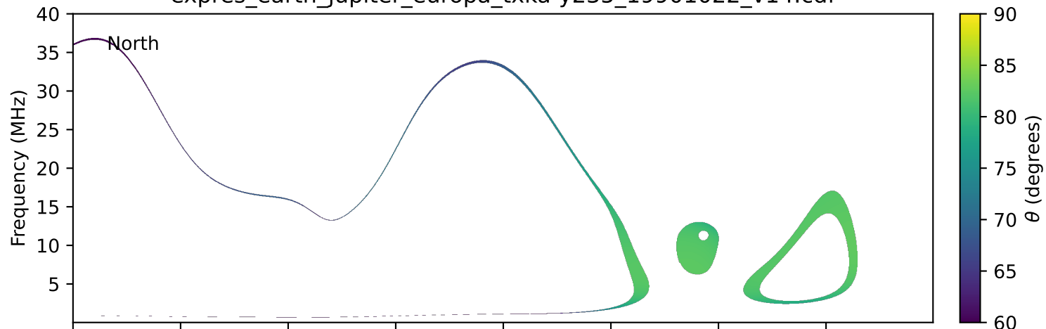
expres_earth_jupiter_europa_txka-y235_19901022_v14.cdf
