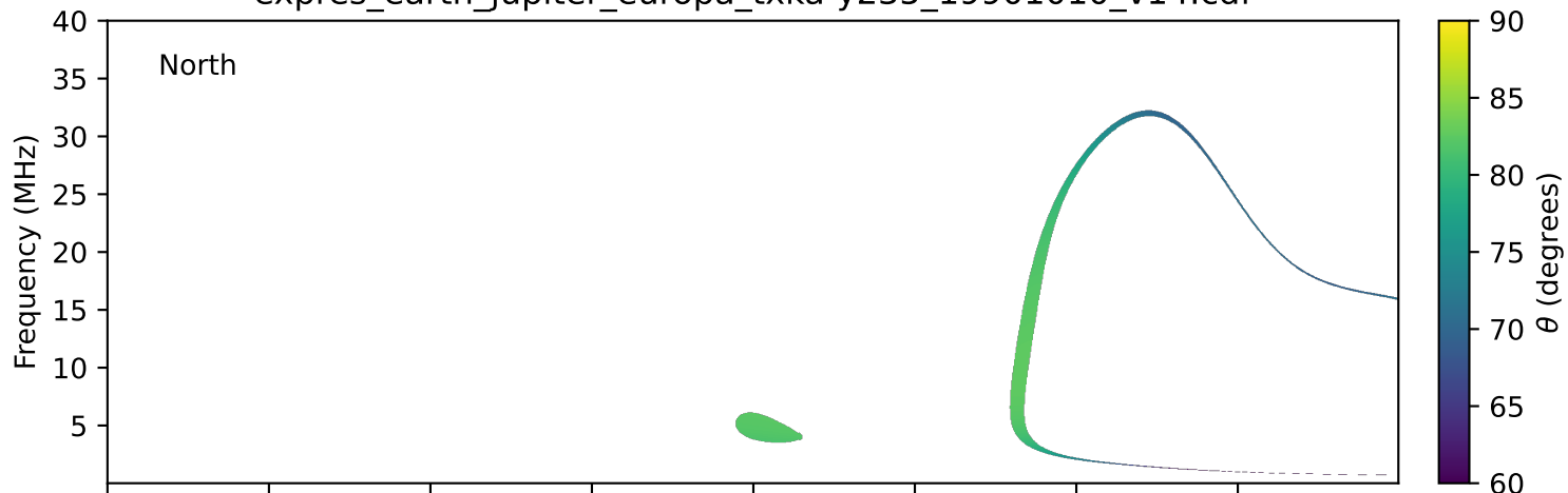
expres_earth_jupiter_europa_txka-y235_19901010_v14.cdf
