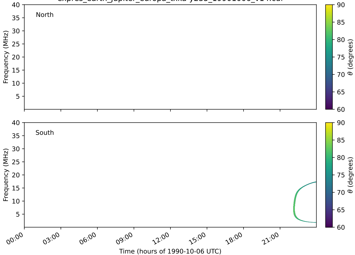
expres_earth_jupiter_europa_txka-y235_19901006_v14.cdf
