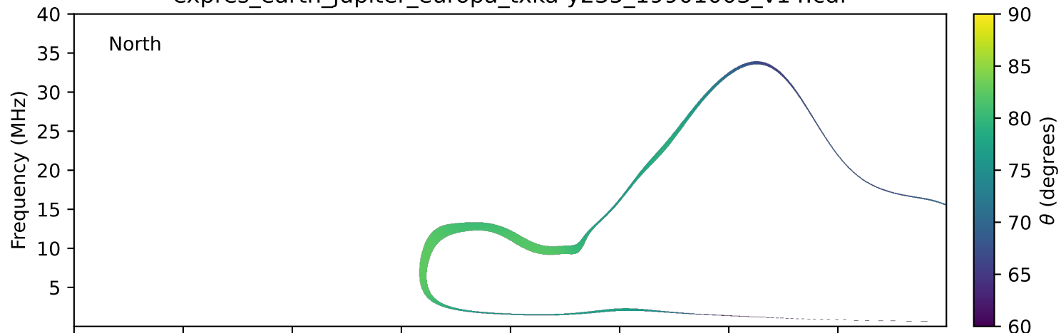
expres_earth_jupiter_europa_txka-y235_19901003_v14.cdf
