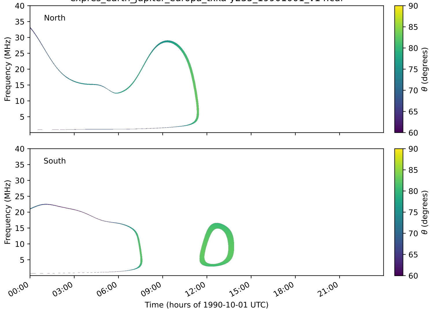
expres_earth_jupiter_europa_txka-y235_19901001_v14.cdf
