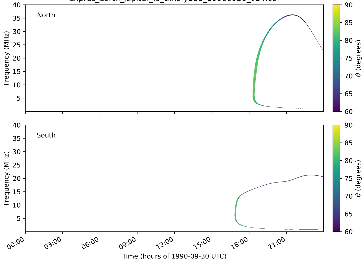
expres_earth_jupiter_io_txka-y235_19900930_v14.cdf
