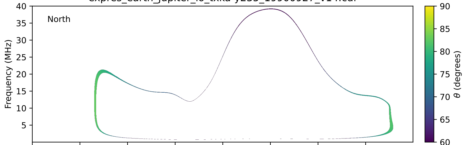
expres_earth_jupiter_io_txka-y235_19900927_v14.cdf
