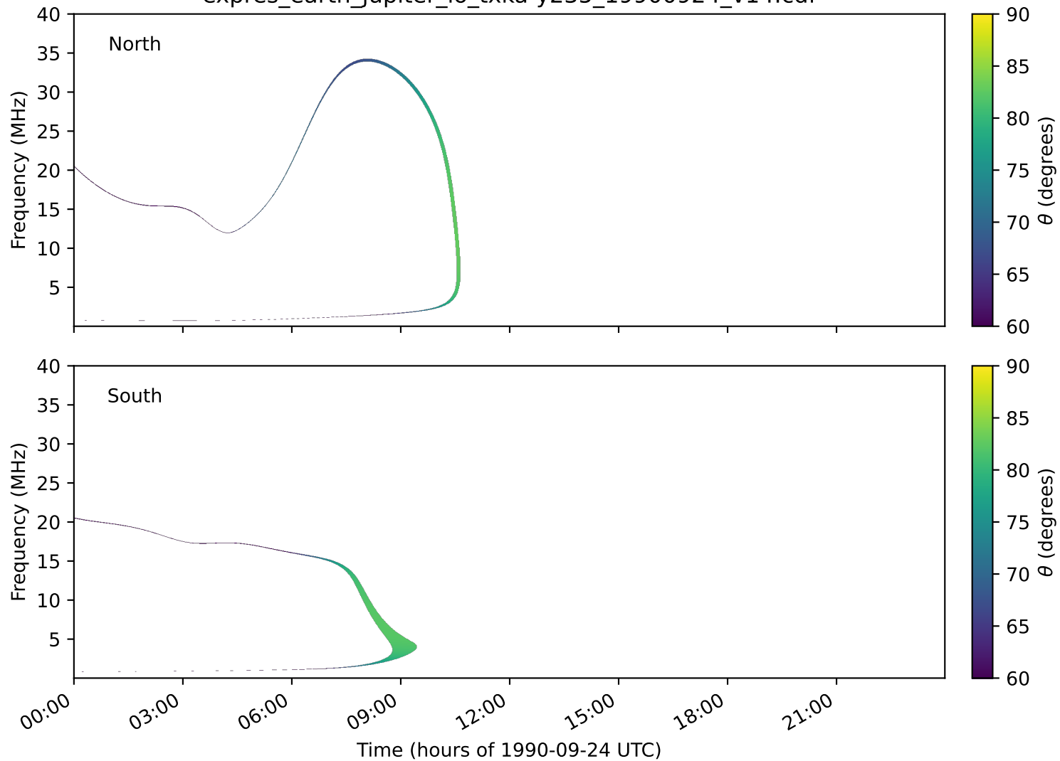
expres_earth_jupiter_io_txka-y235_19900924_v14.cdf
