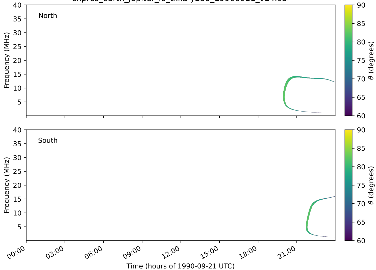
expres_earth_jupiter_io_txka-y235_19900921_v14.cdf
