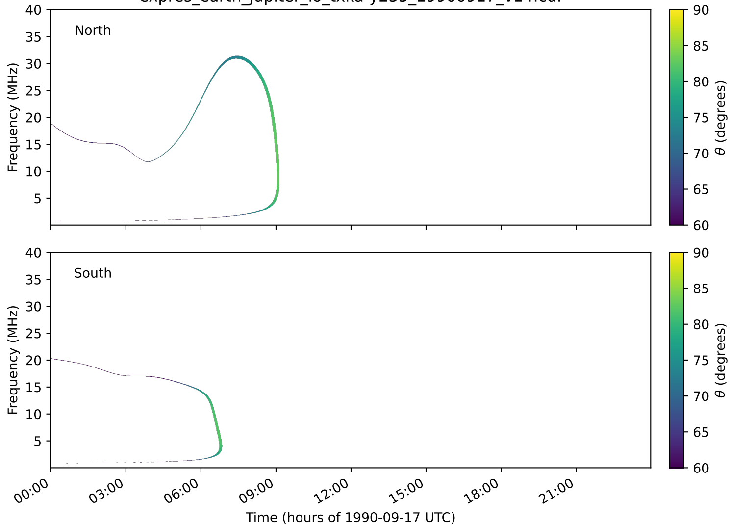
expres_earth_jupiter_io_txka-y235_19900917_v14.cdf
