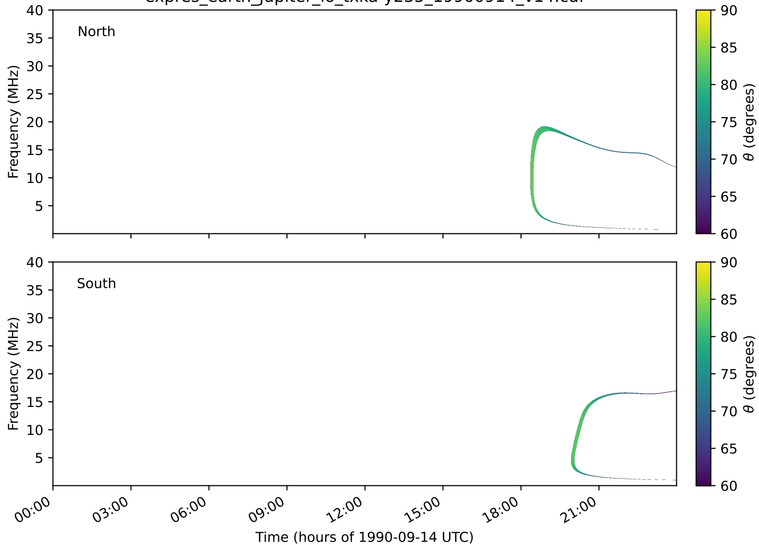
expres_earth_jupiter_io_txka-y235_19900914_v14.cdf
