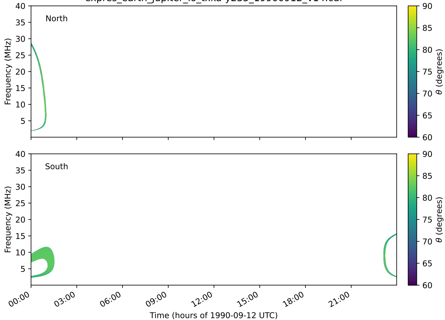
expres_earth_jupiter_io_txka-y235_19900912_v14.cdf
