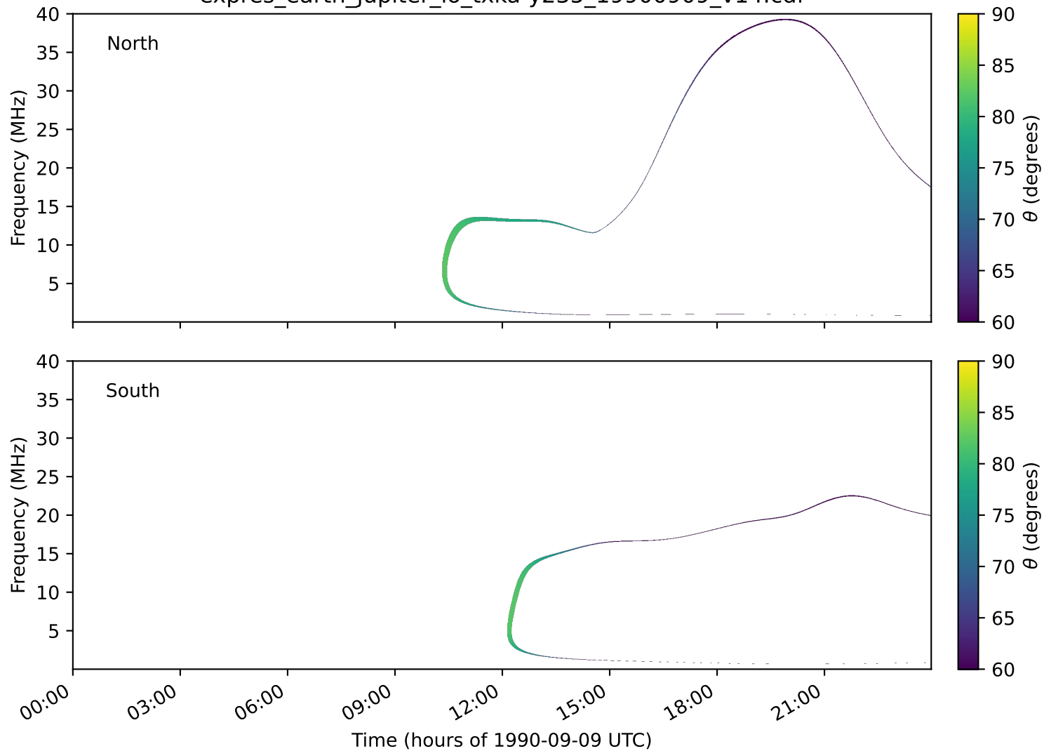
expres_earth_jupiter_io_txka-y235_19900909_v14.cdf
