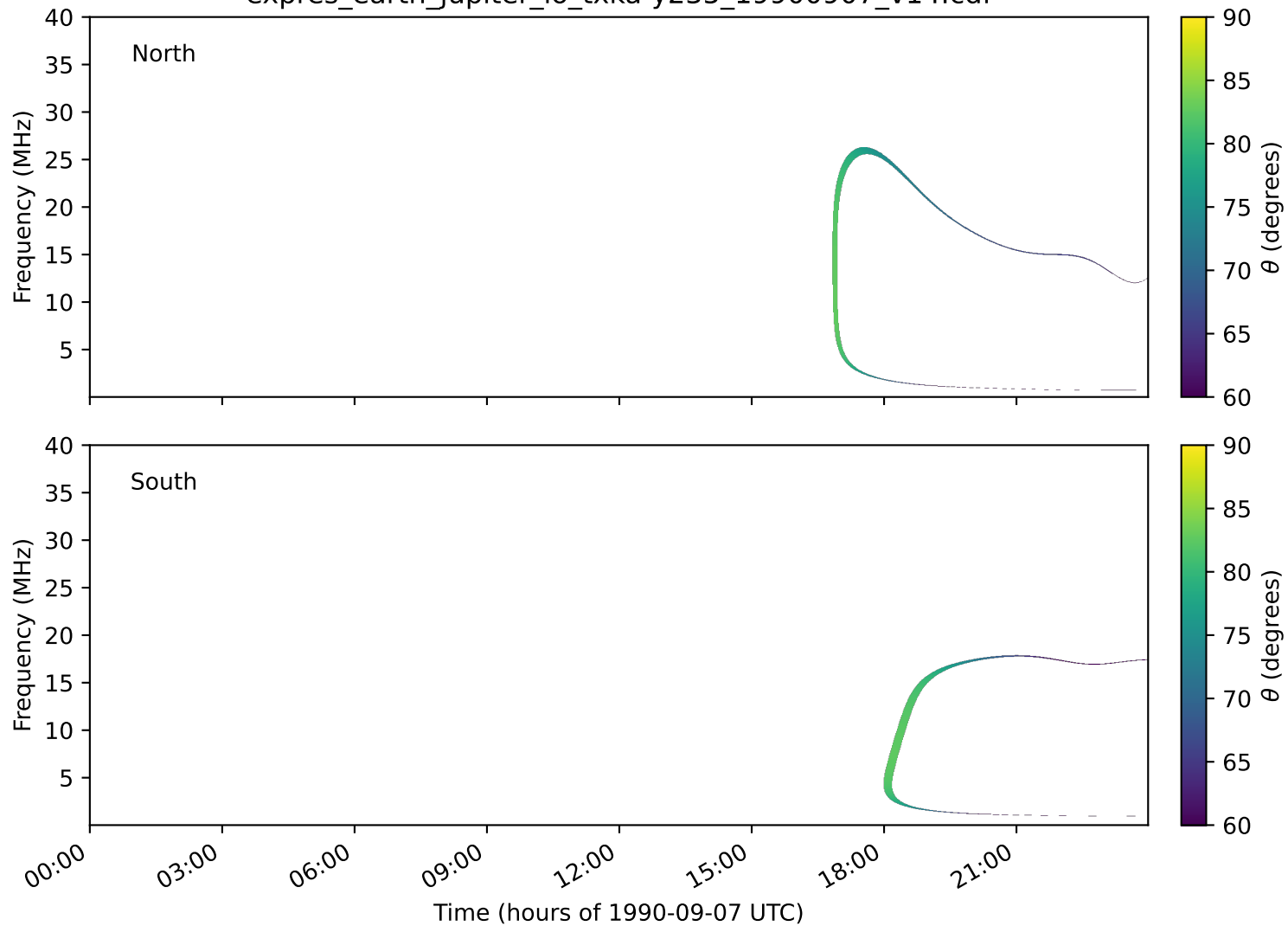
expres_earth_jupiter_io_txka-y235_19900907_v14.cdf
