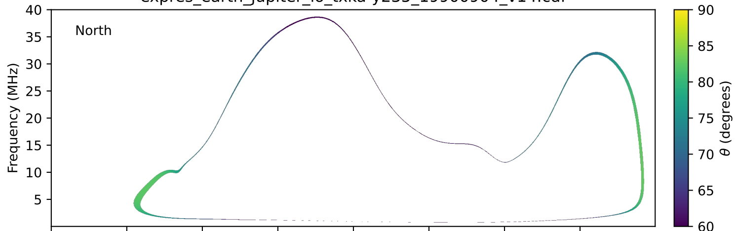
expres_earth_jupiter_io_txka-y235_19900904_v14.cdf
