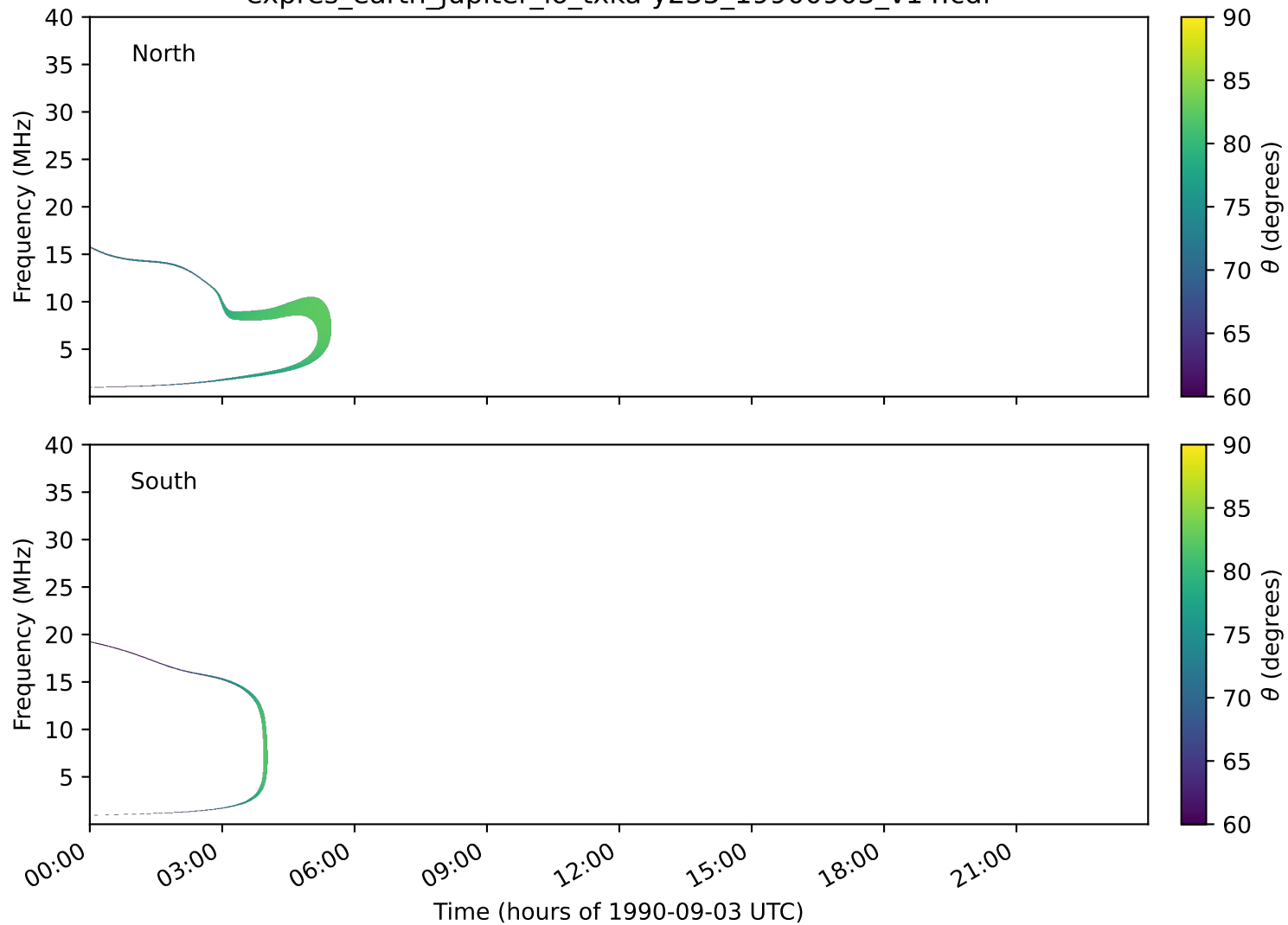
expres_earth_jupiter_io_txka-y235_19900903_v14.cdf
