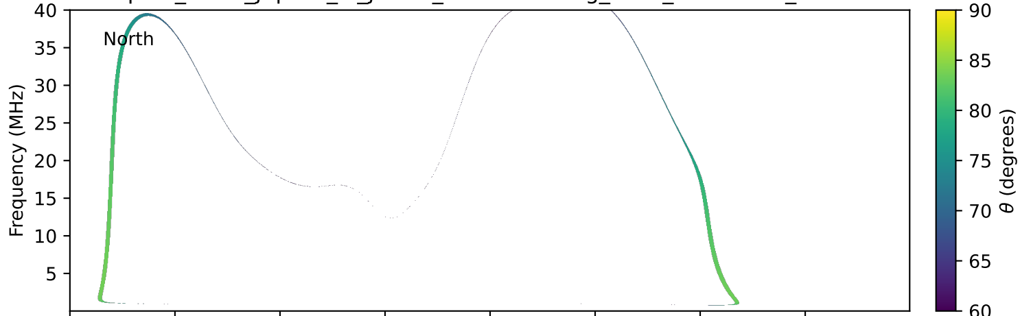
expres_earth_jupiter_io_jrm33_lossc-wid1deg_3kev_19900913_v11.cdf
