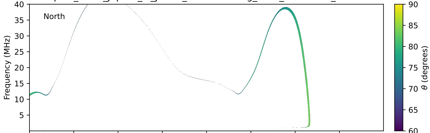
expres_earth_jupiter_io_jrm09_lossc-wid1deg_3kev_19900929_v11.cdf
