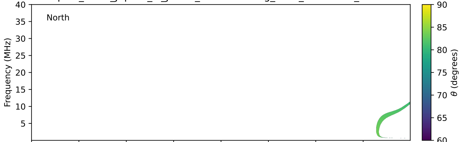
expres_earth_jupiter_io_jrm09_lossc-wid1deg_3kev_19900928_v11.cdf
