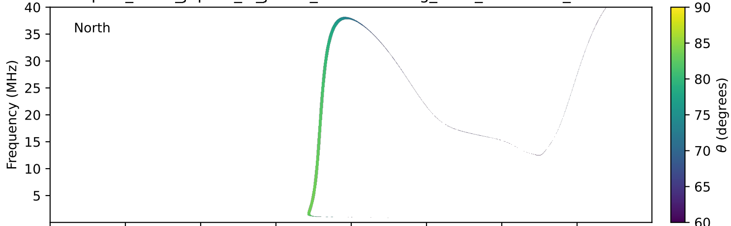
expres_earth_jupiter_io_jrm09_lossc-wid1deg_3kev_19900925_v11.cdf
