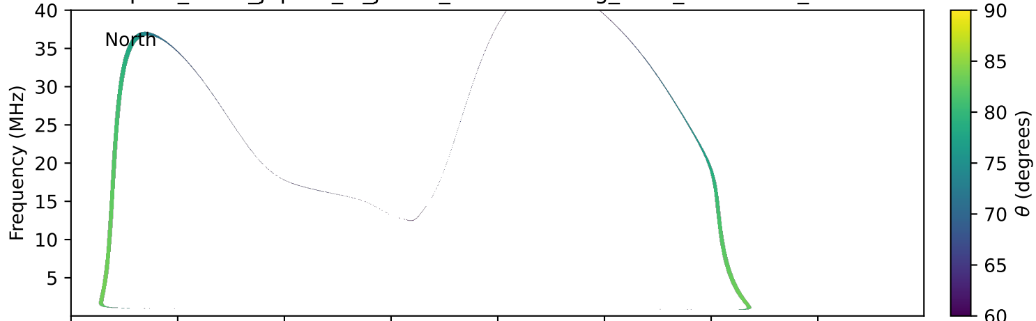
expres_earth_jupiter_io_jrm09_lossc-wid1deg_3kev_19900913_v11.cdf
