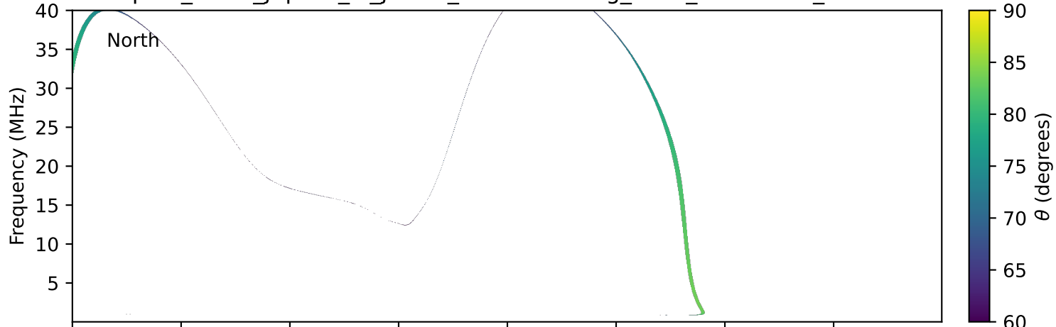
expres_earth_jupiter_io_jrm09_lossc-wid1deg_3kev_19900906_v11.cdf
