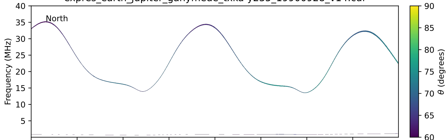
expres_earth_jupiter_ganymede_txka-y235_19900928_v14.cdf
