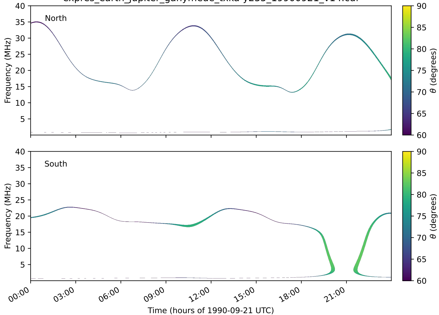
expres_earth_jupiter_ganymede_txka-y235_19900921_v14.cdf
