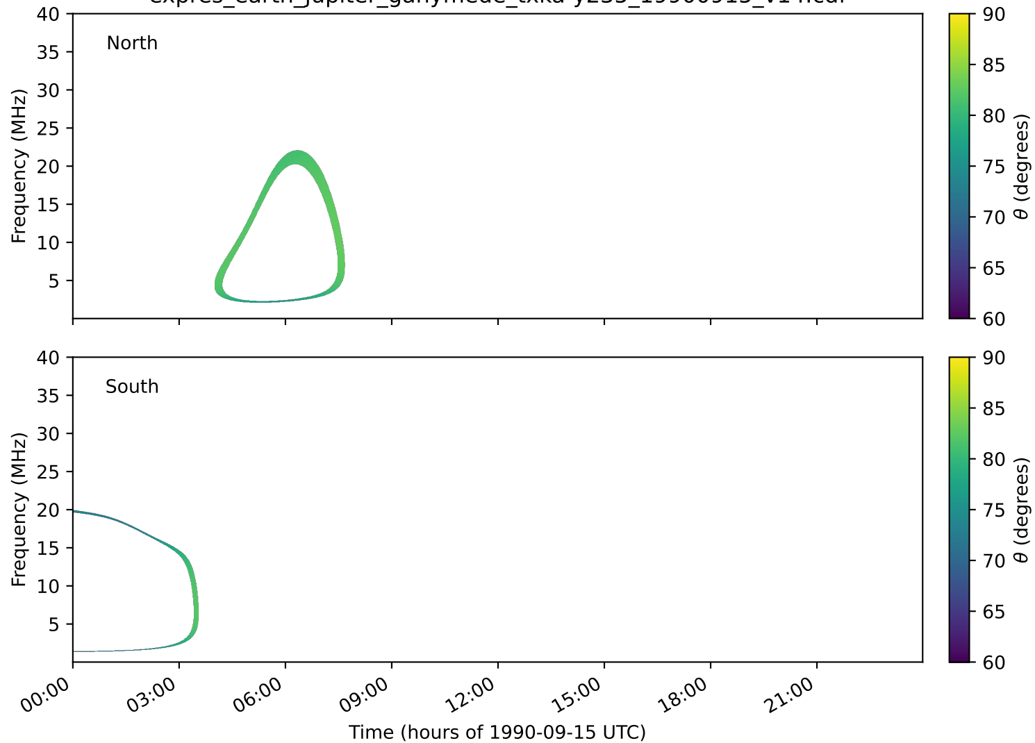
expres_earth_jupiter_ganymede_txka-y235_19900915_v14.cdf
