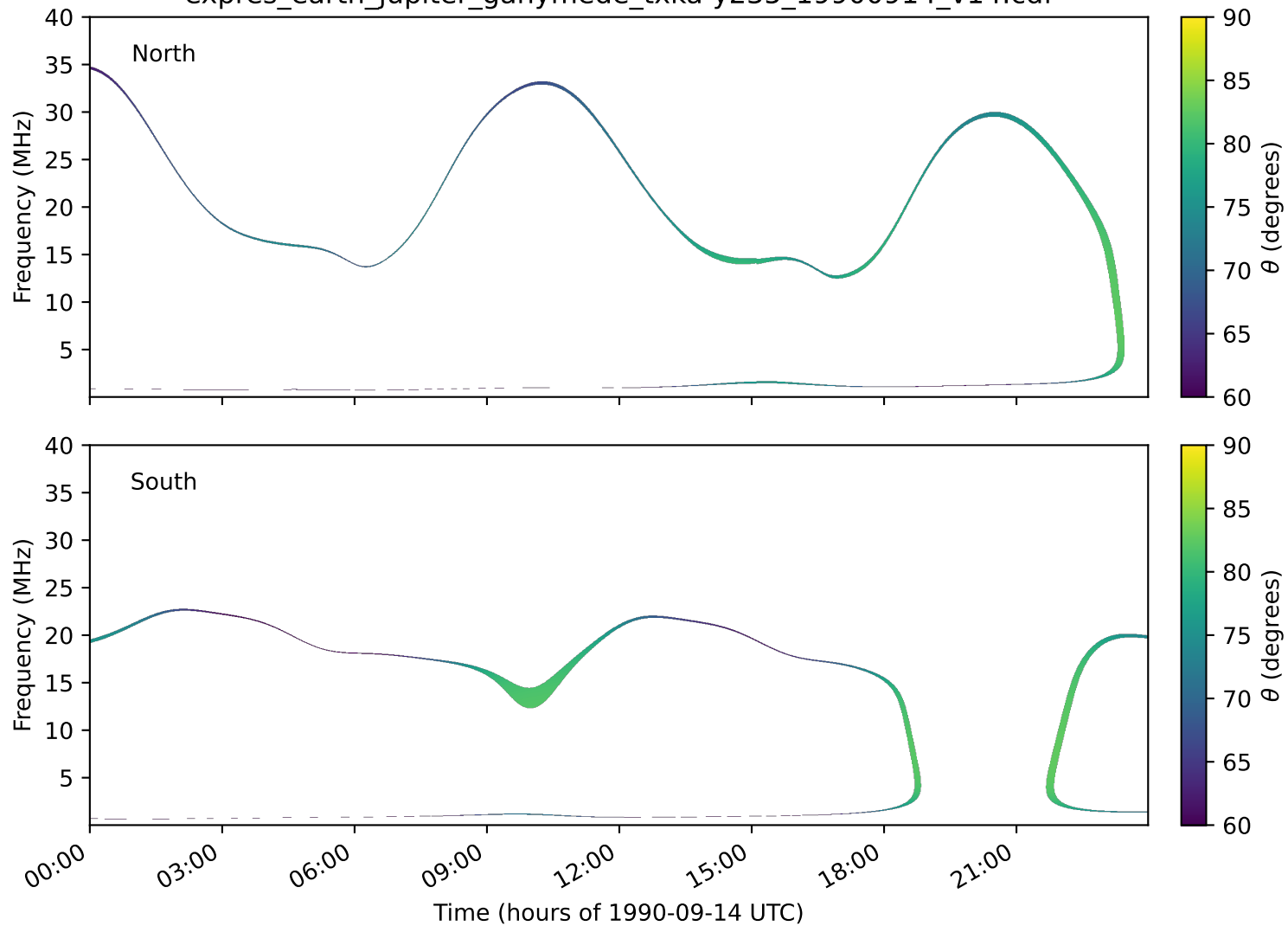
expres_earth_jupiter_ganymede_txka-y235_19900914_v14.cdf
