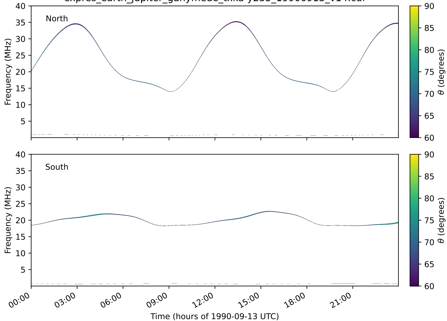
expres_earth_jupiter_ganymede_txka-y235_19900913_v14.cdf
