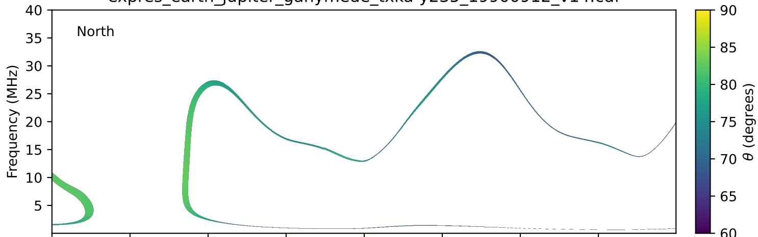
expres_earth_jupiter_ganymede_txka-y235_19900912_v14.cdf
