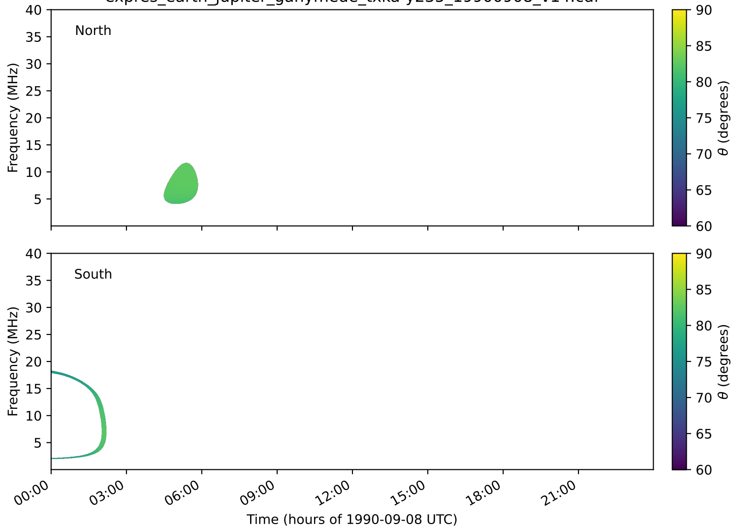
expres_earth_jupiter_ganymede_txka-y235_19900908_v14.cdf
